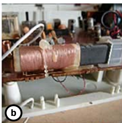
b Ferrite rod antenna in an AM radio
