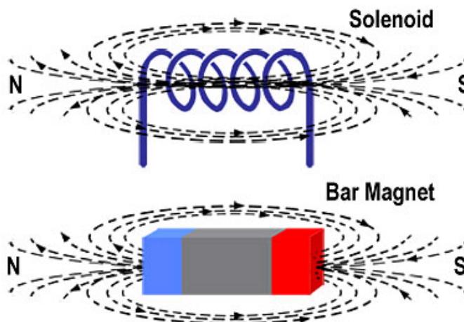
Fig. 3.1.5 Magnetic Field Around a Solenoid and a Bar Magnet.
