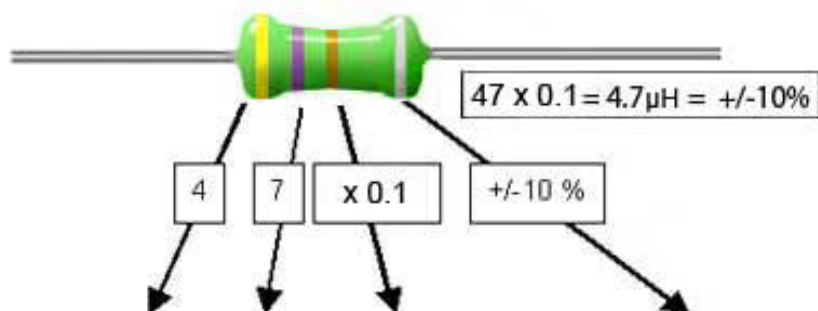
Fig 3.4.1 Four Band Standard E I A Colour Code For Inductors.
