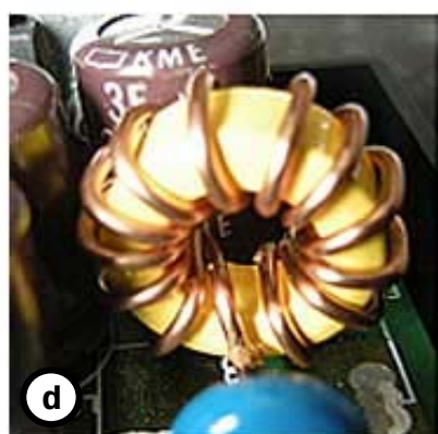
d High current Toroidal Inductor in a power supply
