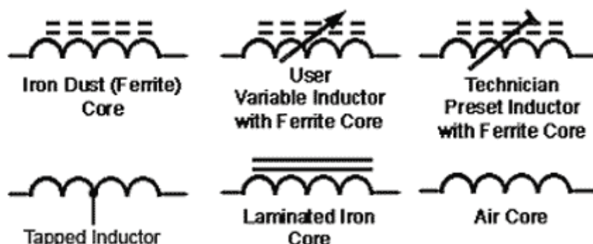
Fig. 3.3.3 Inductor (Schematic) Circuit Symbols.
