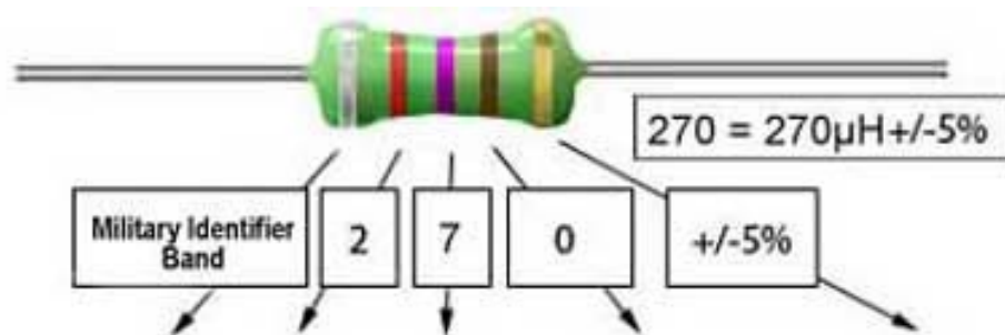
Fig 3.4.2 Five Band Military Standard Inductor Colour Code
