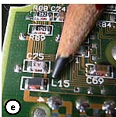
e Surface Mount inductor in a Hard Disk Drive. Typical values can be 0.1nH – 220nH
