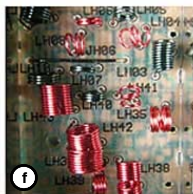
f Air Cored inductors in a TV tuner working at UHF may have very few turns
