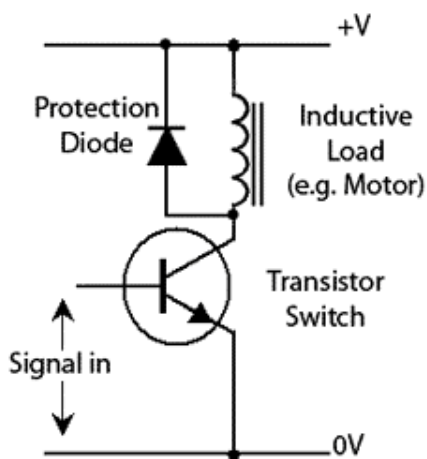
Fig. 3.2.2 Back e.m.f. Protection
