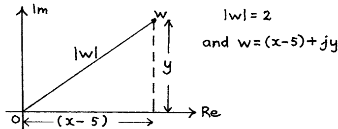
Argand diagram for w
