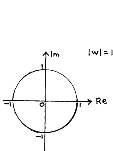
Argand diagram for w
