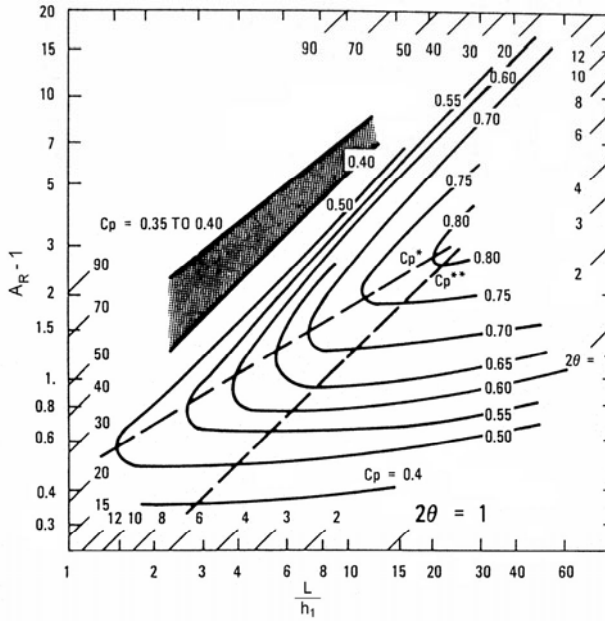
Fig. 1.18. Pressure recovery in plane diffusers (inlet boundary layer blockage 1.5%) [1.8]. Note that (A_R - 1) is plotted on the ordinate.
