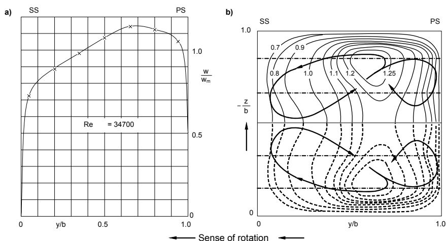
Fig. 5.4. Rotating channel of quadratic section, SS Suction side, PS pressure side, [5.3] a velocity distribution in the direction of the channel axis. b Constant-velocity curves and secondary flow
