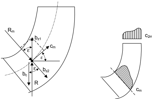
Fig. 5.8. Accelerations and velocities acting in the meridional section
