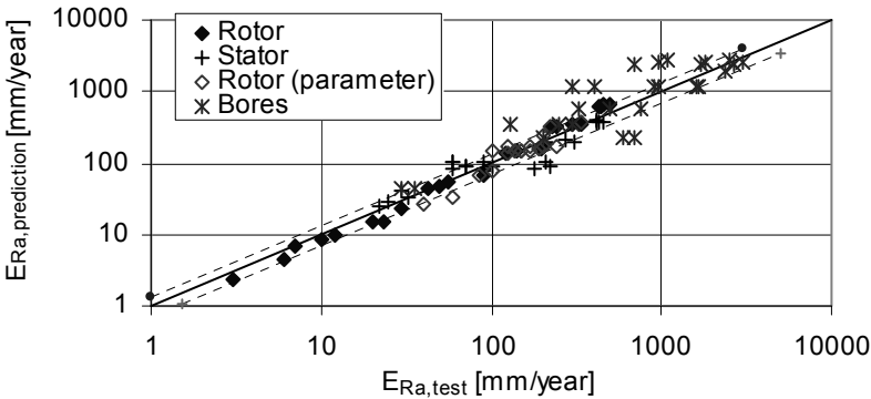
Fig. 14.22. Comparison of test data with prediction according to Table 14.21; rotor/stator: X105CrCoMo 18-2, H_{\text{Mat}} = 700 \text{ HV} ; bores in duplex steel H_{\text{Mat}} = 212 \text{ HV}
