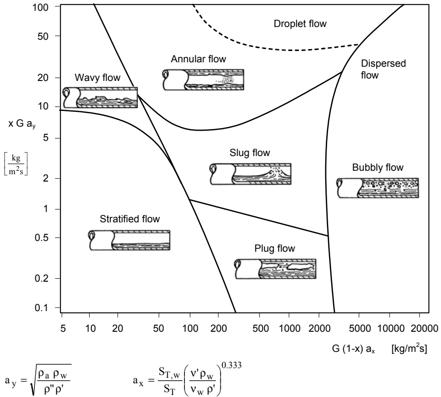
Fig. 13.10. Flow patterns in horizontal pipes, according to [13.5]. S_T = surface tension, G = m_{\text{tot}}/A = mass velocity. Subscripts: w = water, a = air at 20°C and 1 bar.
