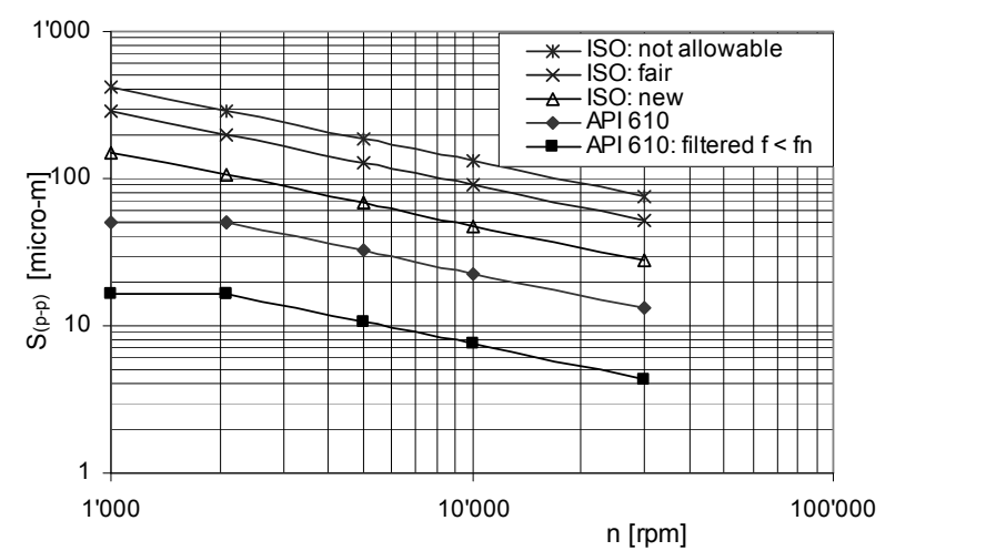
Fig. 10.28. Shaft vibration limits, unfiltered peak-to-peak S_{(p-p)} measured on the major orbit axis; ISO 7919-3 and ISO 13709 (API 610 unfiltered and filtered)
