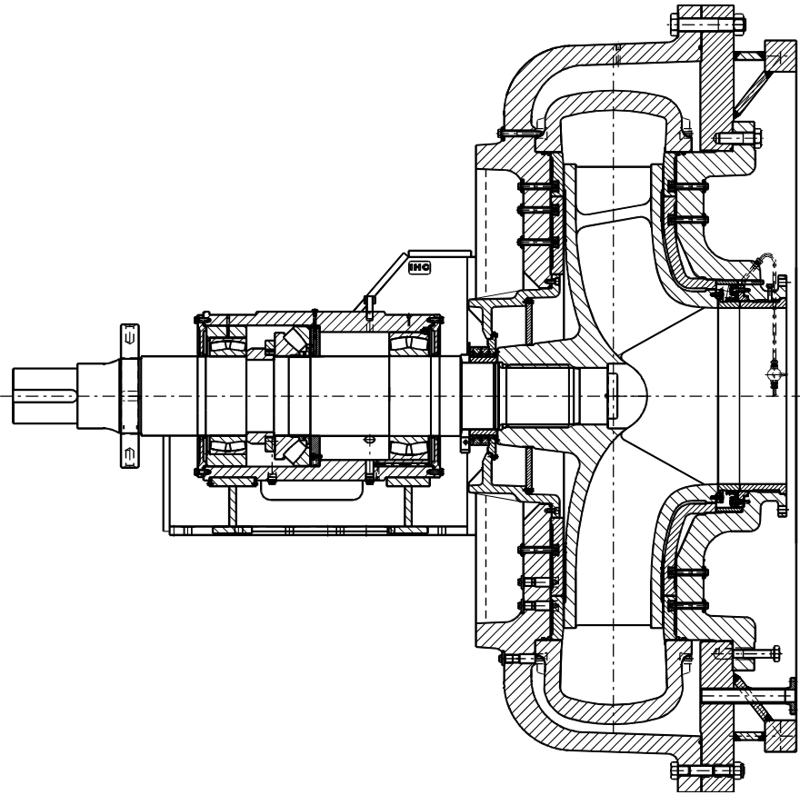
Fig. 13.33. Double-walled dredge pump, d_2 = 2600 mm, n = 240 rpm, Q_{\text{opt}} = 3.5 m 3 /s, H_{\text{opt}} = 67 m, n_q = 19 ; IHC Holland
