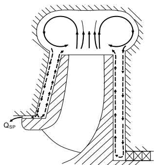
Fig. 9.3. Influence of secondary flows in the volute on the impeller sidewall gaps
