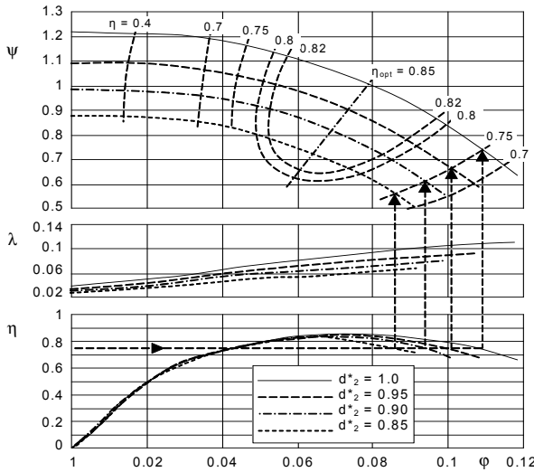
Fig. 4.18. Determination of constant-efficiency curves (note that all pressure coefficients are referred to the full impeller diameter); d_2^* = d_2'/d_2
