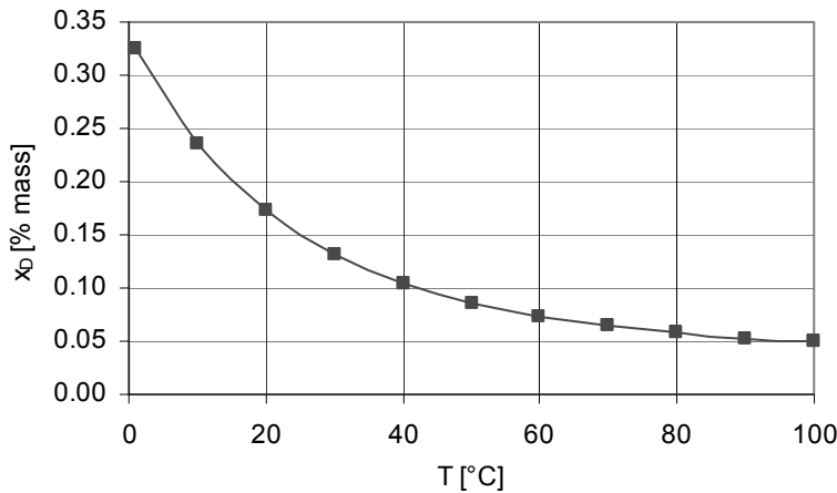
Fig. A3.3. Solubility in mass per cent of \text{CO}_2 in water at a partial pressure of 1.013 bar
