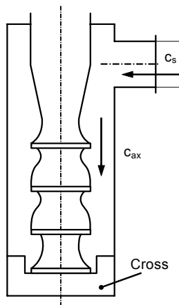
Fig. 11.26. Approach flow to can pumps
