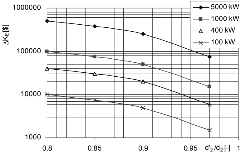
Fig. 4.21. Additional energy costs caused by efficiency impairment due to trimming; valid for volute pumps, calculated with k_{kW} = 2000 $/kW, \eta_o = 0.8 and \varepsilon = 0.2 . Enter the graph with the combined power of all trimmed pumps ( z_{pp} \times P ), where P is the power of one pump. Example: The impellers of 4 pumps in parallel, each with a power of 250 kW, are to be trimmed by 10%; the total power consumption is thus z_{pp} P = 1000 kW. With d'_2 = 0.9 read from curve “1000 kW” the additional capitalized energy costs of 50'000 $. If the costs of a new pattern or a pattern modification are below this amount, it is economical to invest in new patterns. This would also make sense with respect to material costs and ecology.
