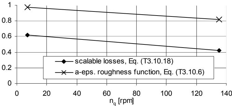
Fig. 3.31. Weighting the roughness a_e acc. to Eq. (T3.10.6) and fraction of scalable losses acc. to Eq. (T3.10.18): a_e = 0.98 - 0.0012 n_q f_q^{0.5}
