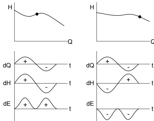
Fig. 11.12. Dynamic instability
