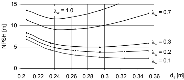
Fig. 7.1. Optimization of the impeller inlet diameter d_i
