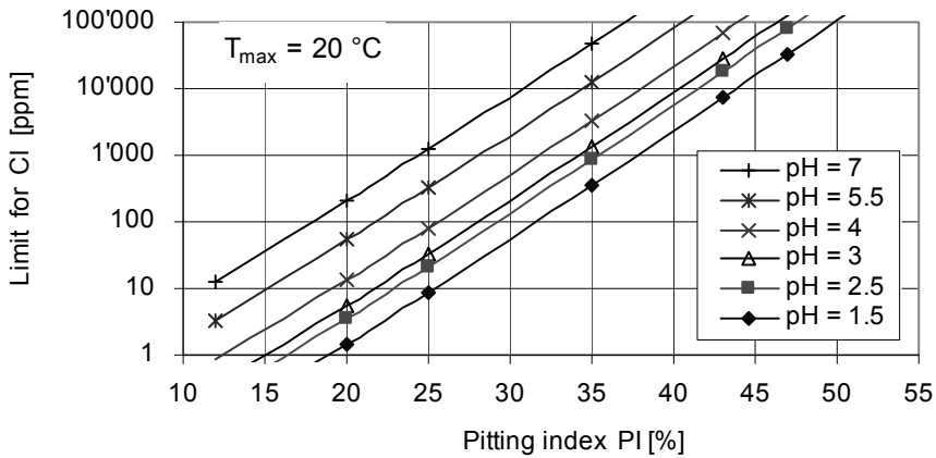
Fig. 14.17. Limits for the chloride content as a function of pitting index and pH; valid for T < 20^\circ\text{C} .
