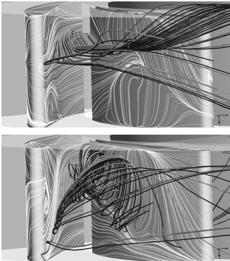
Fig. 5.42. Flow patterns in a diffuser of a pump with double-entry impeller, diffuser and volute, q^* = 0.8 , CFD calculations [5.52].
