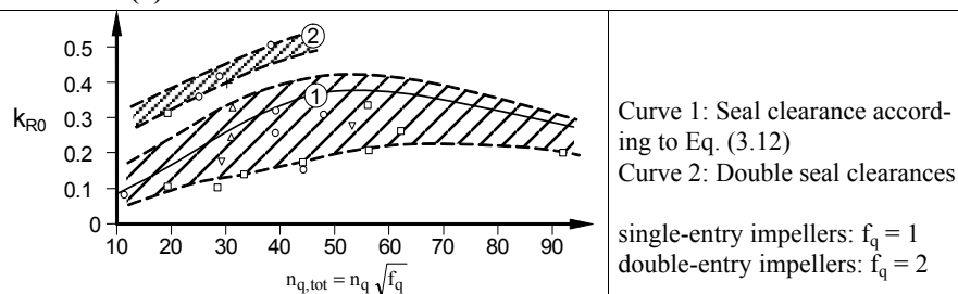
Fig. 9.27. Static radial force coefficients for single volutes at shut-off ( Q = 0 )
