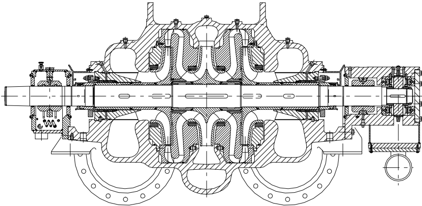
Fig. 2.12. Two-stage, double-entry water transport pump, Sulzer Pumps n = 1490 \text{ rpm} , Q_{\text{opt}} = 1.7 \text{ m}^3/\text{s} , H_{\text{opt}} = 465 \text{ m} , P_{\text{opt}} = 8600 \text{ kW} , \eta_q = 23
