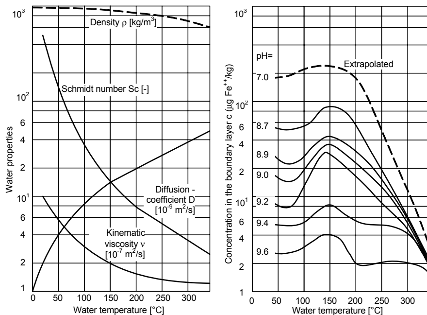
Fig. 14.14. Properties of water and solubility of magnetite, conditioned with ammonia, \text{O}_2 -content less than 20 to 40 ppb, parameter: pH at 25°C
