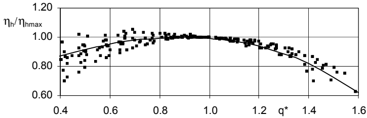
Fig. 4.16. Dependence of hydraulic efficiency \eta_h on the flow rate ratio
