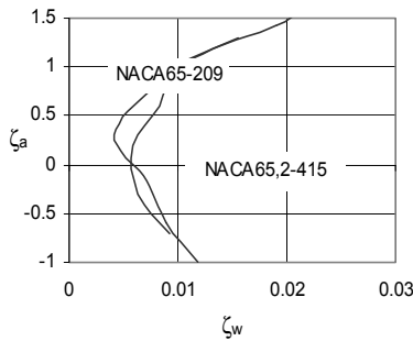
Fig. 7.29. Polar diagram for NACA65-209 and NACA65,2-415, Re = 6 \times 10^6
