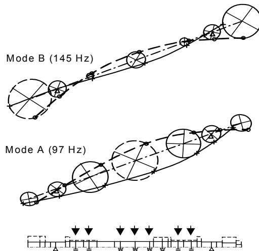
Fig. 10.13. Calculated eigen values and eigen modes, n = 7900 rpm
