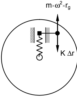
Fig. 1.7. Movement of a point mass on a curved path
