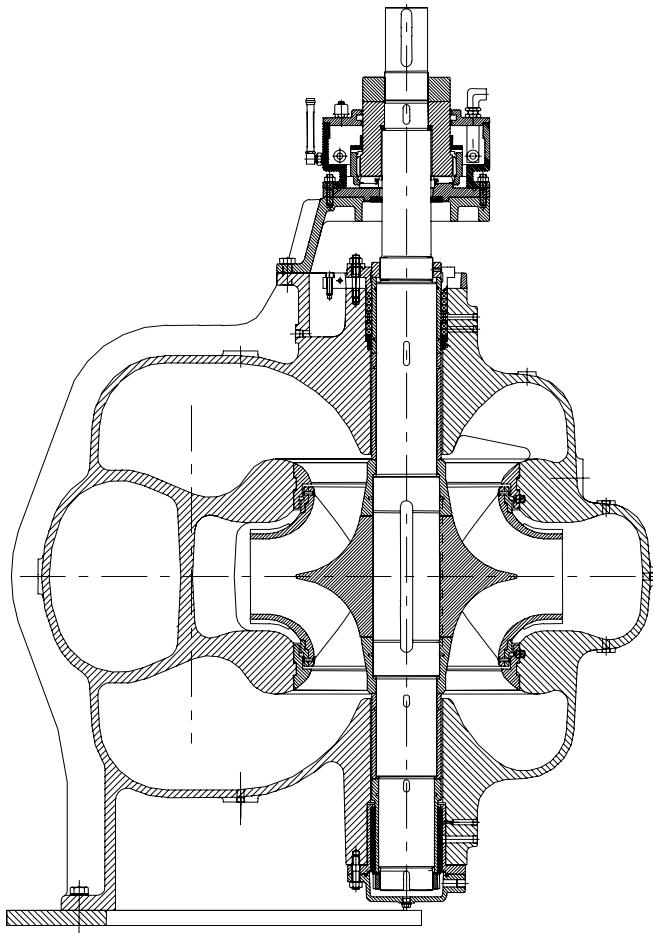
Fig. 2.5. Double-entry vertical pump, Sulzer Pumps, n = 596 rpm, Q_{\text{opt}} = 2.4 \text{ m}^3/\text{s} , H_{\text{opt}} = 48 \text{ m} , P_{\text{opt}} = 1250 \text{ kW} , n_q = 36
