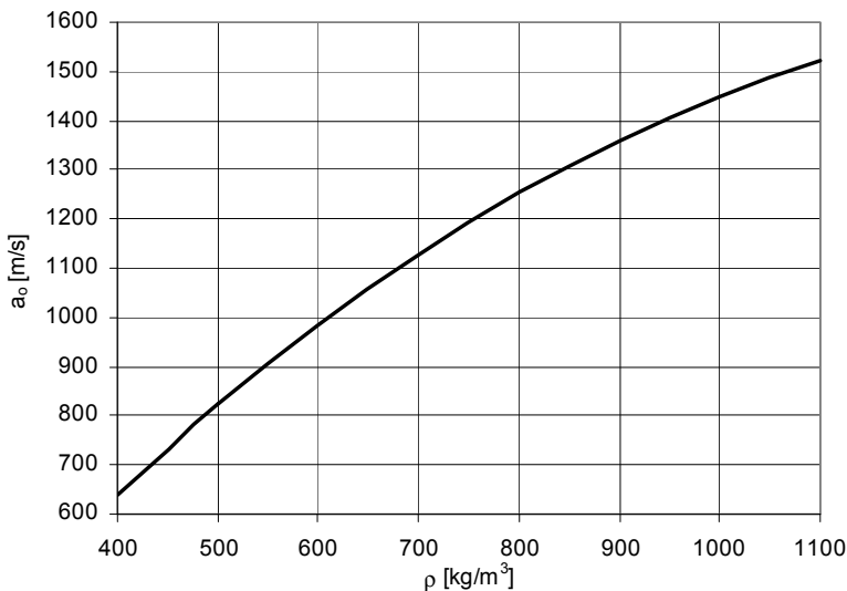
Fig. A5.1. Sound velocity a_0 estimated from liquid density \rho
