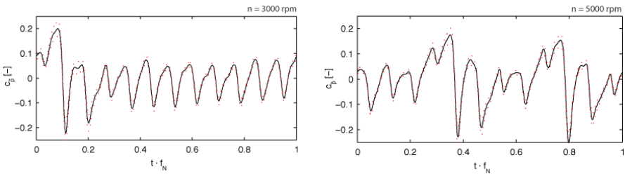
Fig. 10.20. Measured pressure pulsations on a rotating impeller, z_{Le} = 12 , q^* = 0.9 ; left: n = 3000 rpm; right: n = 5000 rpm; [10.67]
