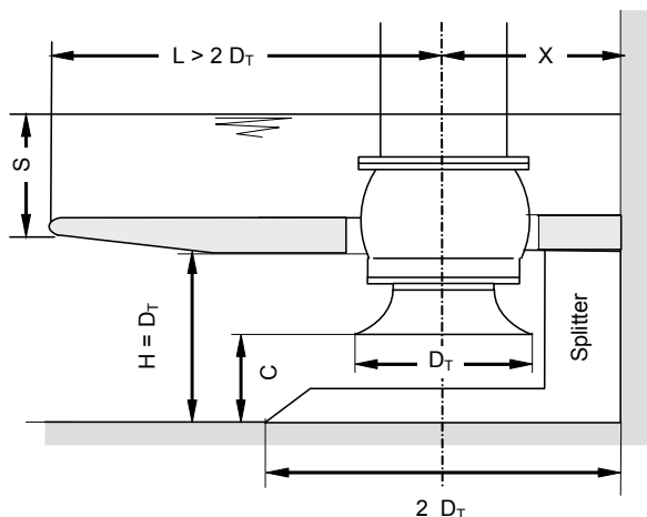
Fig. 11.25. Covered intake chamber
