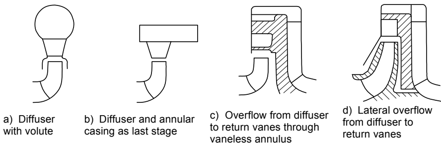
Fig. 7.43. Diffuser arrangements
