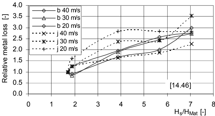
Fig. 14.23. Relative metal loss as function of the hardness; b = bore, j = jet
