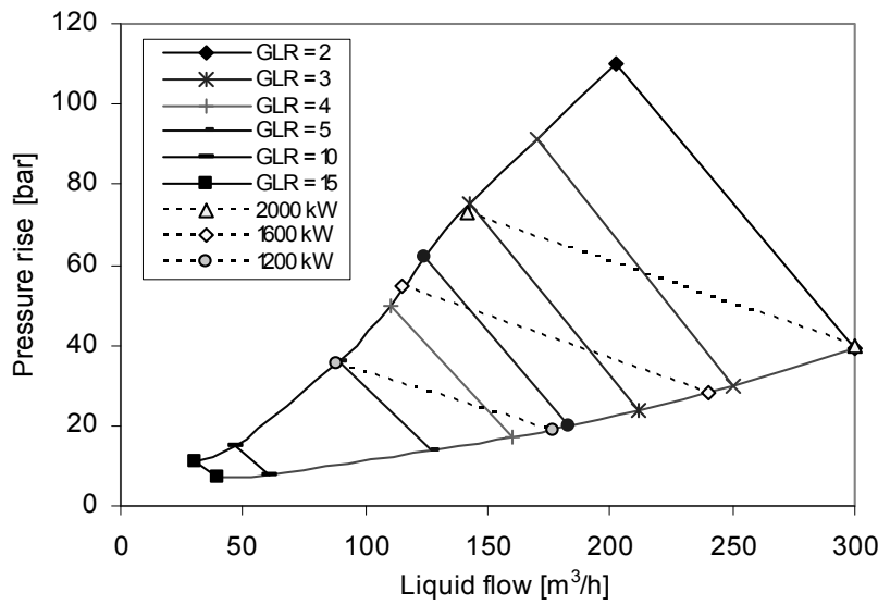
Fig. 13.27. Characteristics of a two-phase pump at constant speed and inlet pressure
