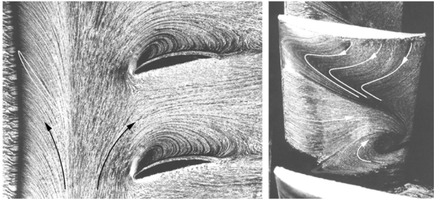
Fig. 5.49. Flow patterns in the diffuser of an axial compressor just prior to the onset of rotating stall; left: flow on the casing wall; right: vane suction side (the hub is at the bottom), [5.46]. Flow is from left to right, rotor moves from bottom to top of the figure.
