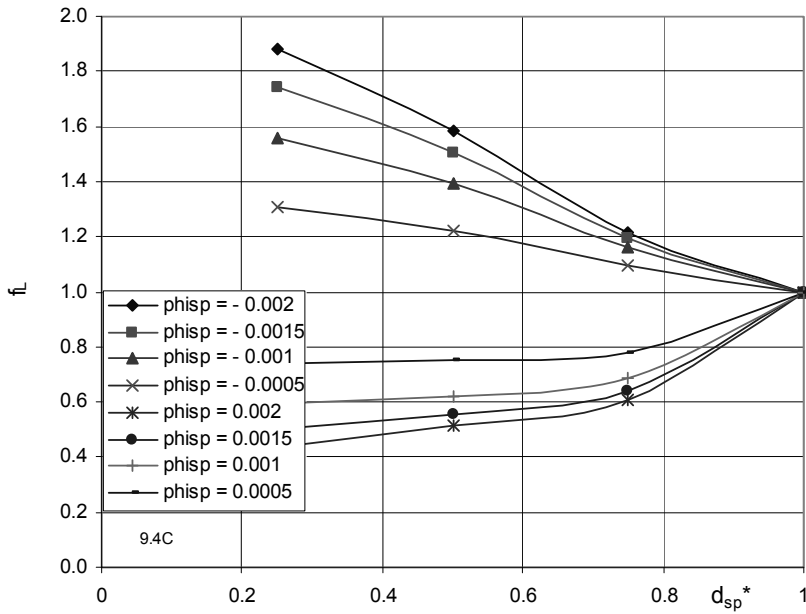
Fig. 9.9. Influence of leakage and seal diameter on disk friction losses, k_E = c_{2u}/u_2 = 0.5
