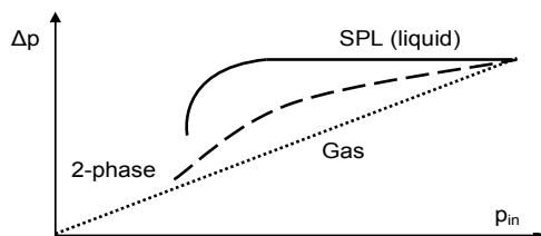
Fig. 13.31. “Suction test” with liquid pump versus two-phase pump and compressor
