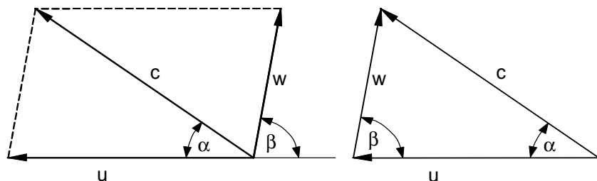
Fig. 1.1. Vector diagram
