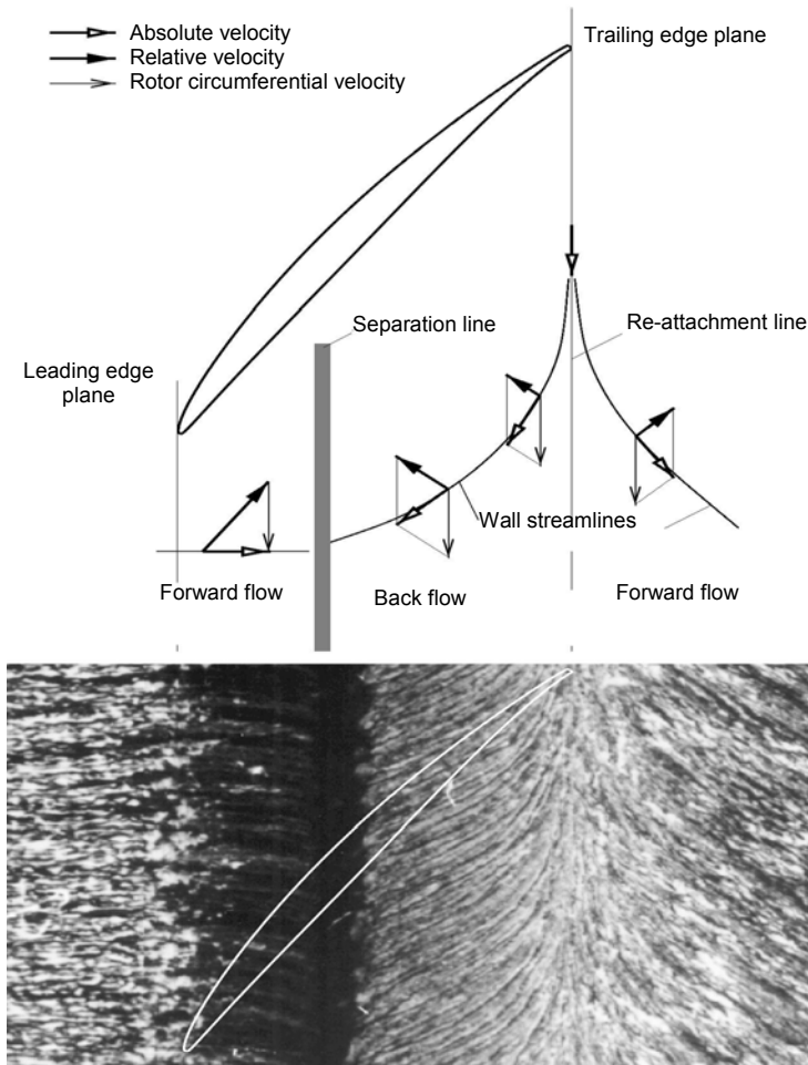
Fig. 5.45. Flow pattern on casing wall; left region: forward flow upstream and near impeller inlet; center region: back-flow within the impeller; right region: forward flow towards diffuser, [5.42]. Flow is from left to right, rotor moves from top to bottom of the figure.
