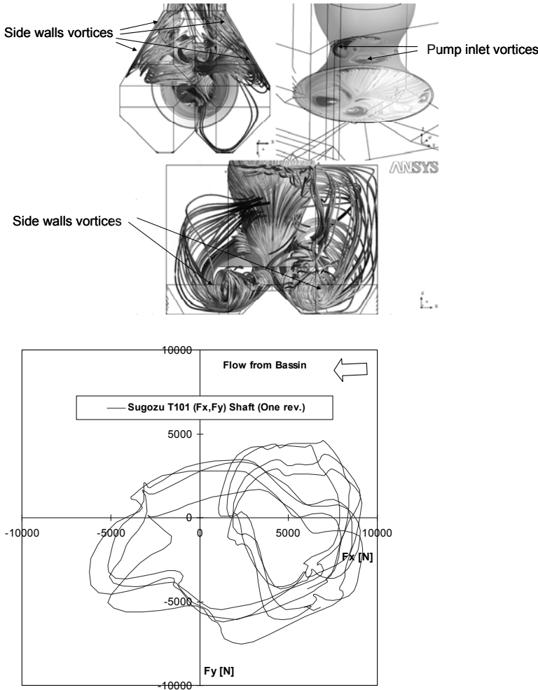
Fig. 9.30. Unsteady radial forces created by the highly distorted approach flow to a semi axial vertical pump, CFD analysis [9.28]
