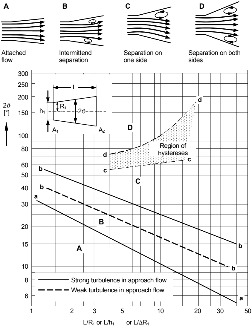
Fig. 1.20. Flow regimes in diffusers
