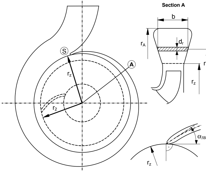
Fig. 3.17. Volute casing
