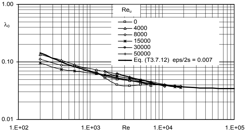
Fig. 3.13. Friction coefficients of smooth annular seals with u_{sp} = 0 according to Fig. 3.11 (eps stands for the sand roughness \epsilon )
