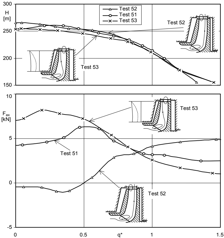
Fig. 5.35. Influence of axial rotor position on Q - H -curve and axial thrust, n_q = 22 , Sulzer Pumps; Test 51: Rotor position centered; Test 52: Rotor shifted to discharge side; Test 53: Rotor shifted to suction side
