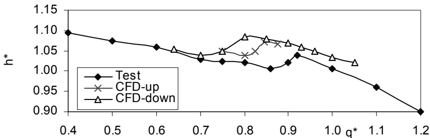
Fig. 8.18. CFD-study of a pump with instable Q-H-curve, h^* = H/H_{opt} , [5.52]
