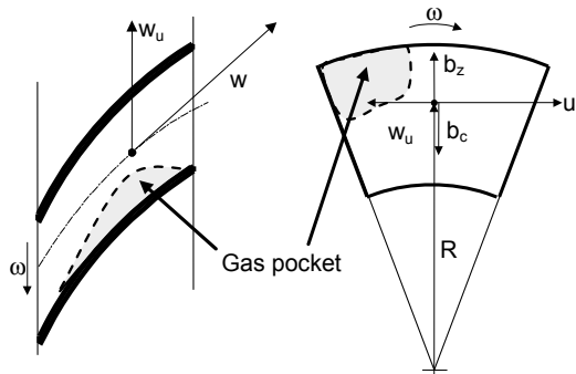
Fig. 13.13. Centrifugal and Coriolis forces in axial or semi-axial impellers and likely locations of gas accumulation
