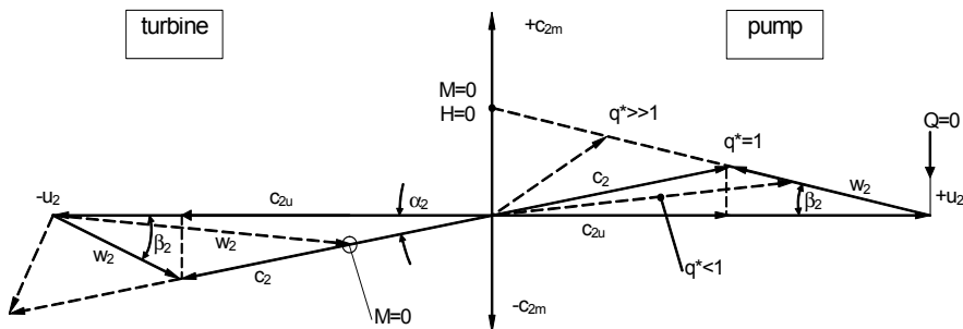
Fig. 12.2. Velocity triangles in pump (right) and in turbine operation (left)
