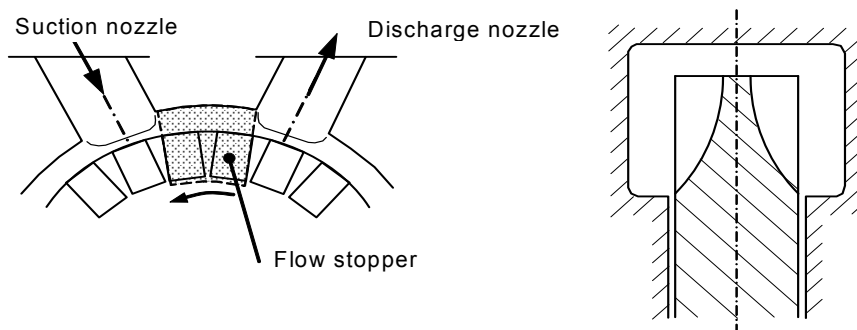
Fig. 2.19. Peripheral pump [2.7]
