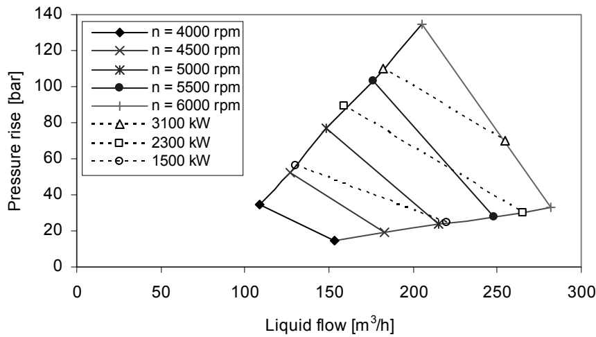
Fig. 13.26. Characteristics of a two-phase pump at constant GVF and inlet pressure
