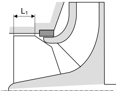
Fig. 7.34. Arranging an inducer in the meridional section
