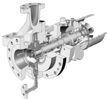
OHH – Overhung Single Stage ISO 13709 (API 610) Type OH2
