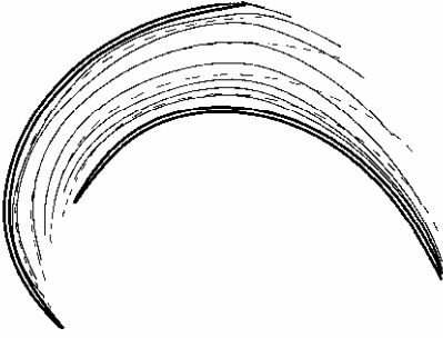
Fig. 3.4. Streamline of relative flow in a radial impeller (Navier-Stokes calculation). The broken lines correspond to blade-congruent flow.
