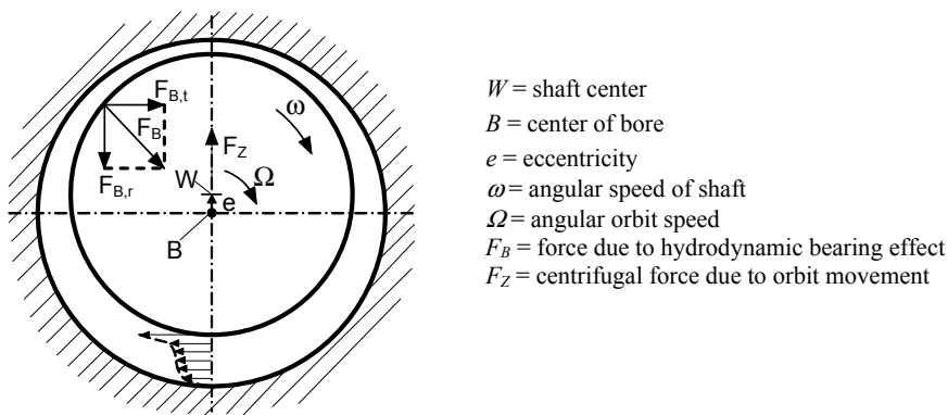
Fig. 10.15. Instability mechanism
