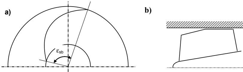
Fig. 7.37. Sweep-back of the inducer blade leading edge
