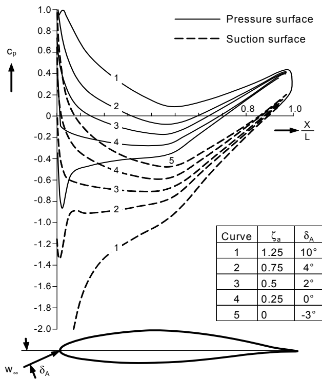
Fig. 7.28. Pressure distribution on airfoil NACA 652-415 according to [7.25]
