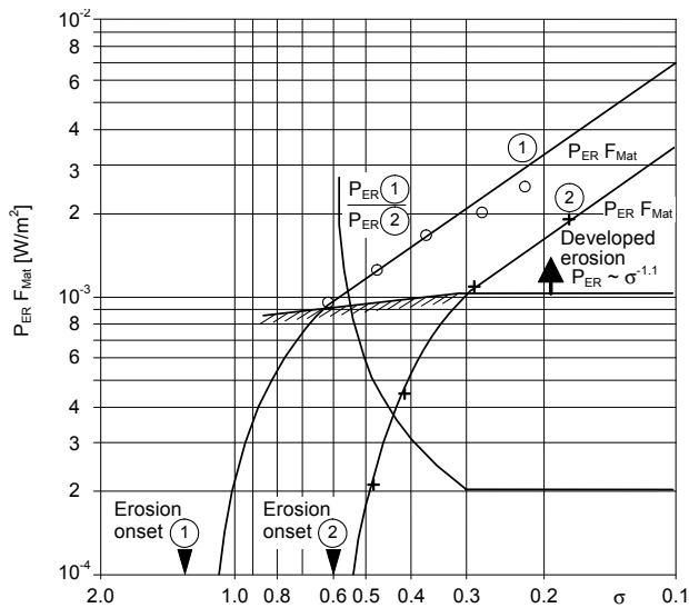
Fig. 6.33. Specific erosion power P_{ER} of two different steels subject to cavitation, [6.20]
