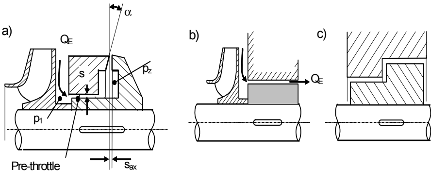
Fig. 9.15. Axial thrust balancing of multistage pumps. a balance disk; b balance piston; c stepped balance piston
