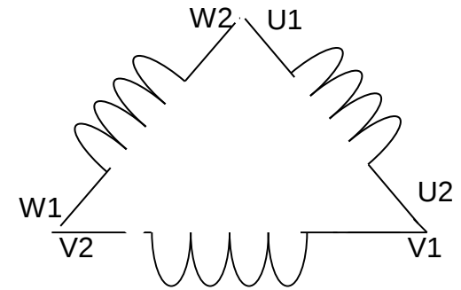
Motor Connections
