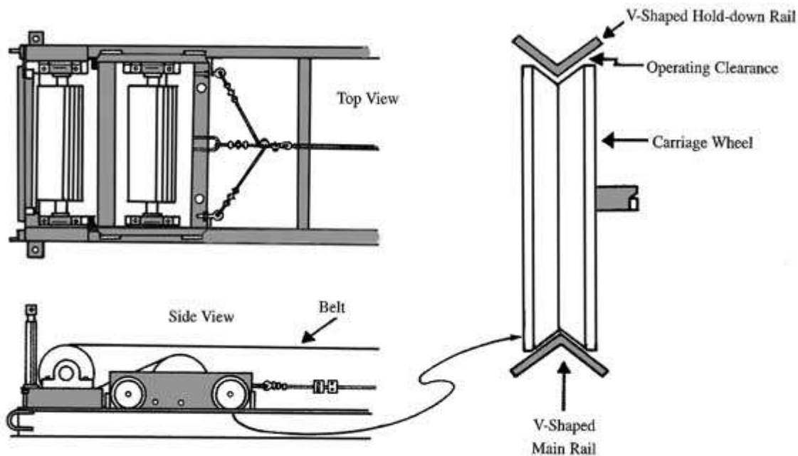
Figure 10 Sample Horizontal Take-Up Carriage
