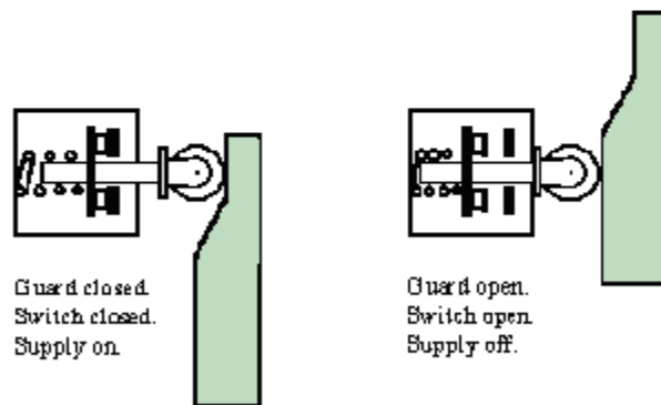
Figure 2. Linear Cam, Positive Switch Actuation (Sliding Guards)
