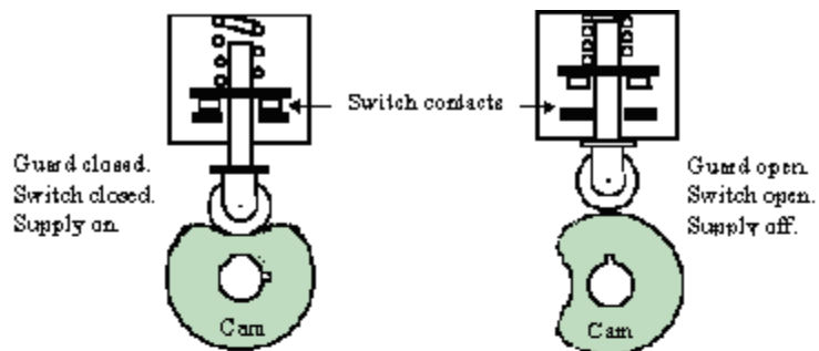
Figure 1. Circular Cam, Positive Switch Actuation (Hinged Guards)
